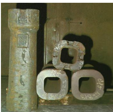
Ingot mould for tube ingot
