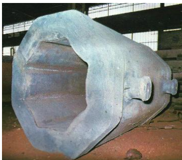
Ingot mould for 40 tons forged ingot
